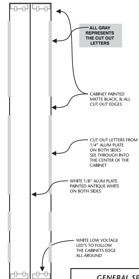
END VIEW
