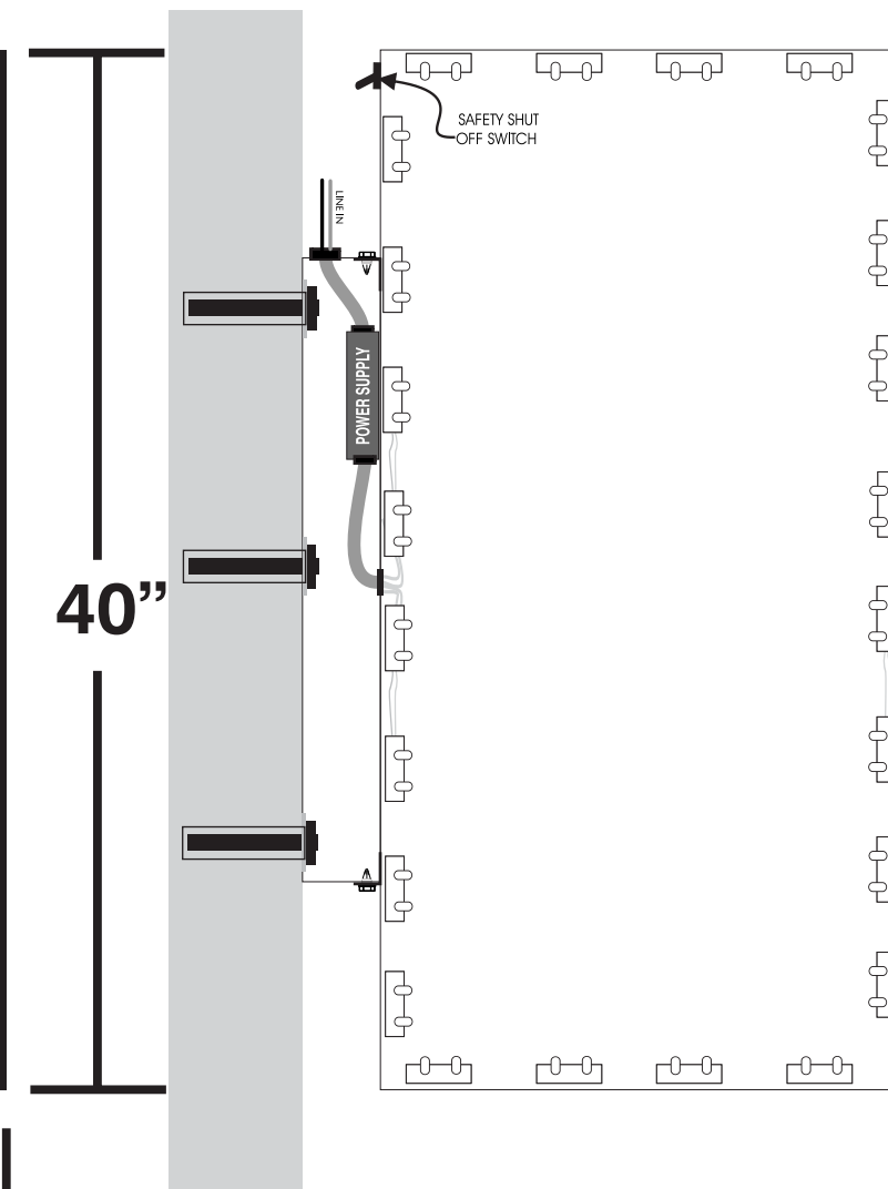
SIDE VIEW MOUNTING
