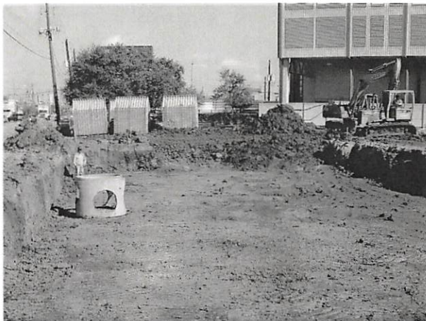
Excavate bed and prepare subgrade per engineer's plans.
