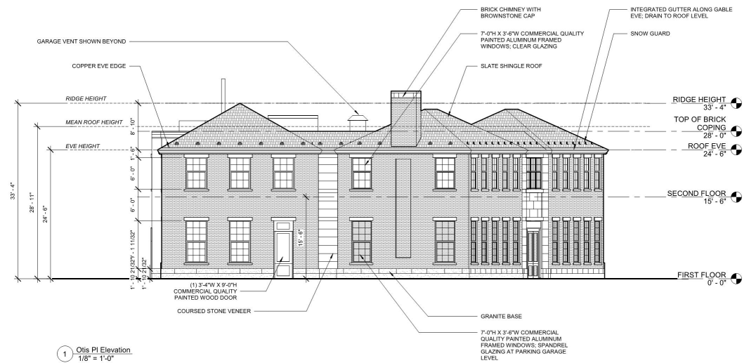
1 Otis Pl Elevation 1/8" = 1'-0"
