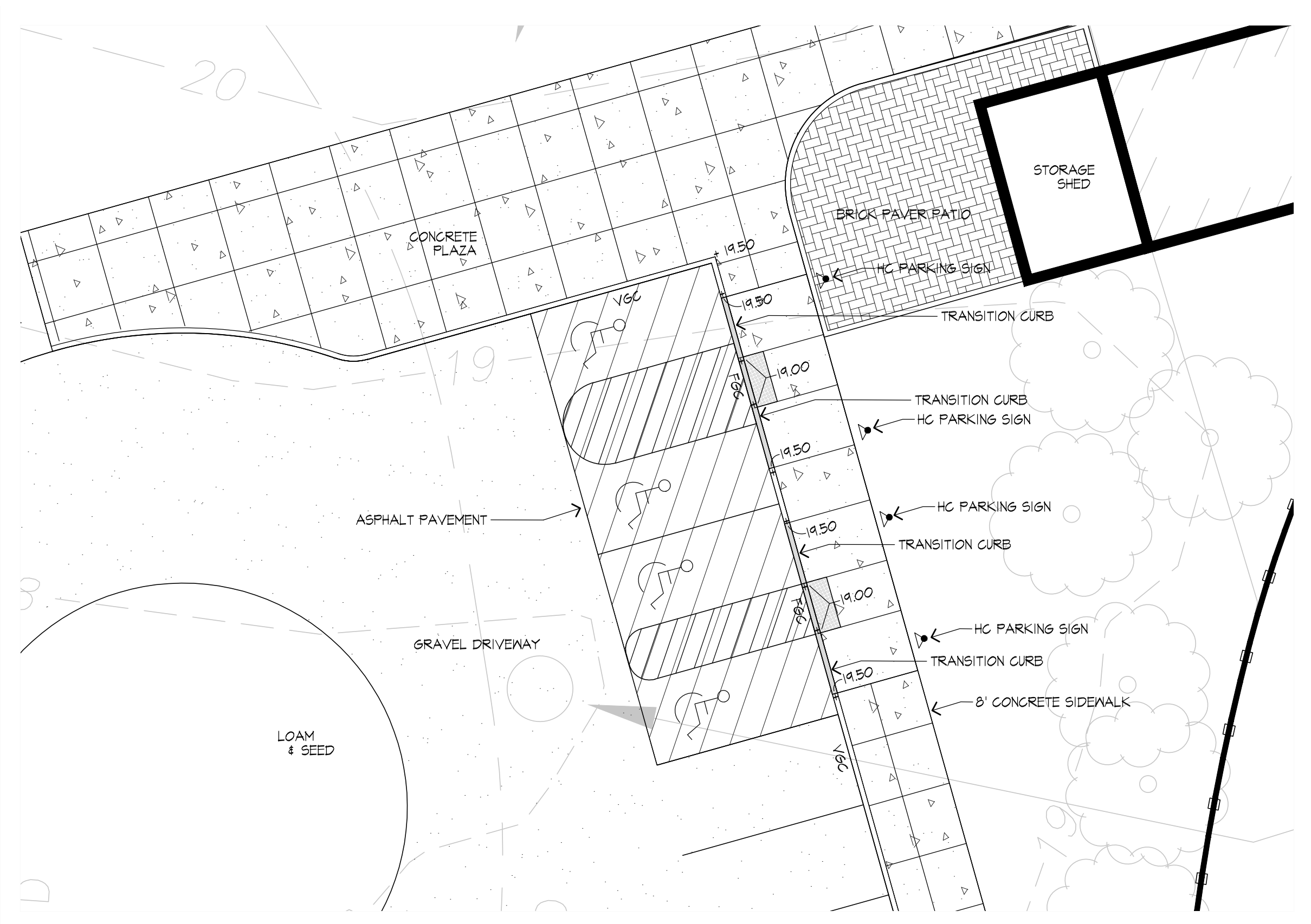
1 HC PARKING ENLARGEMENT SCALE: 1" = 10'
