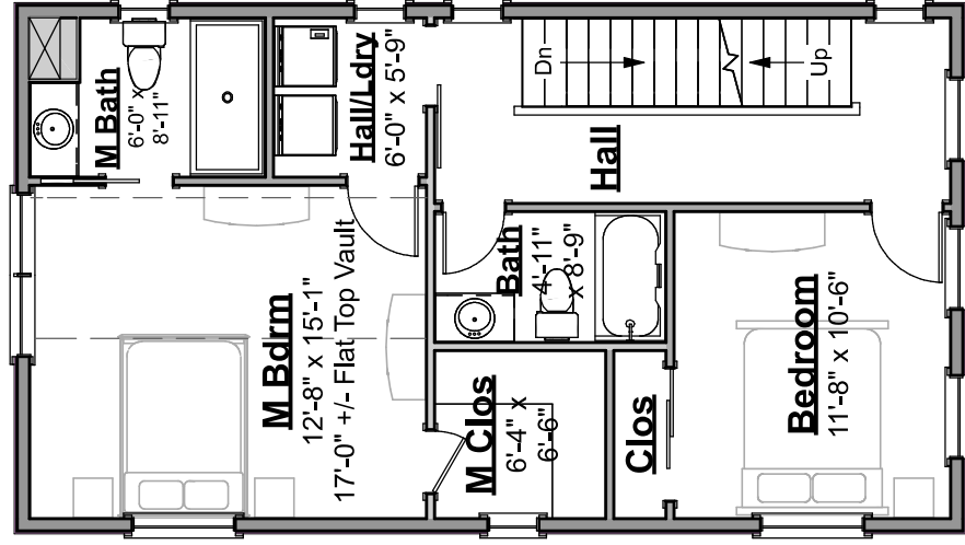
Living Area - Second Floor: 720 sq ft 8 ft Ceilings, unless noted otherwise
