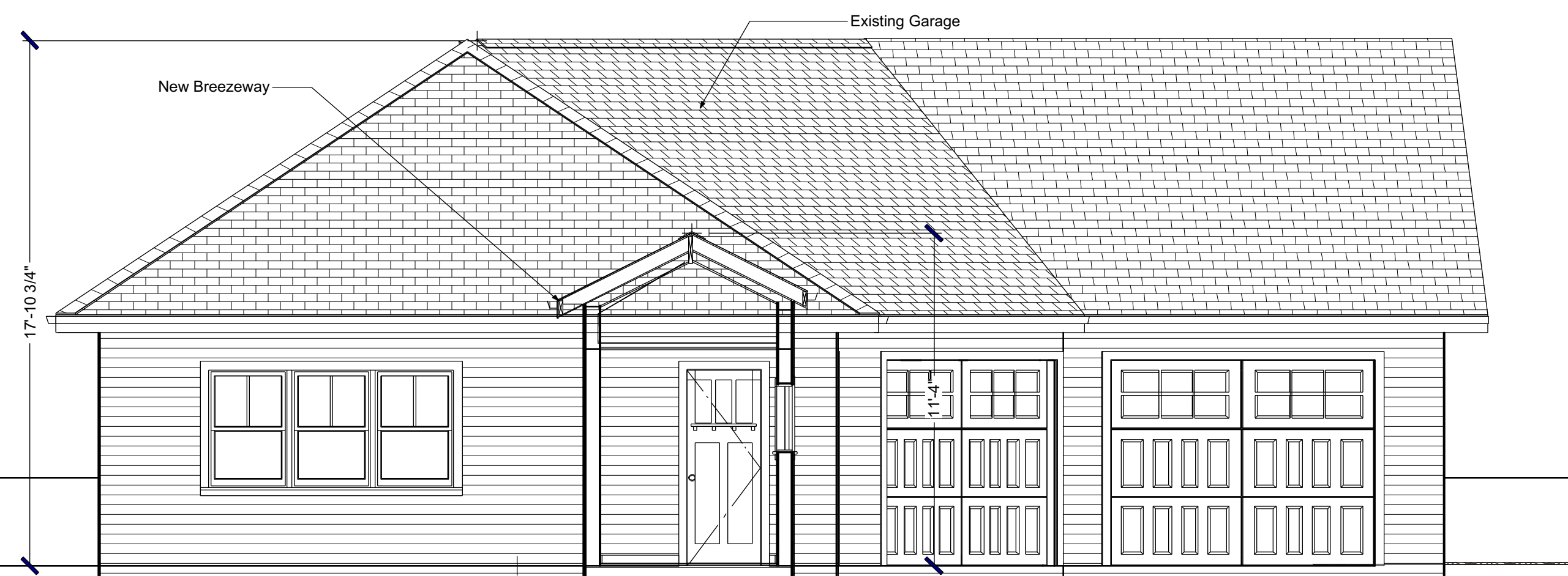
Breezeway section @ Garage
