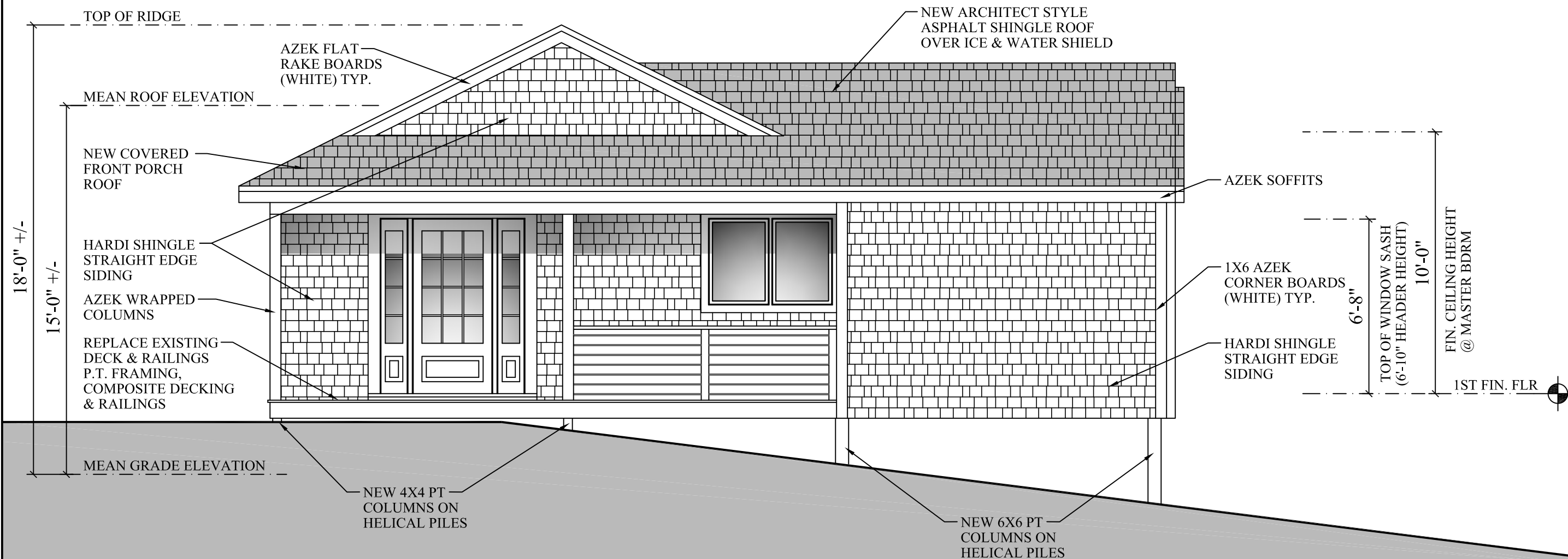
Proposed Southeast Elevation 1/4" = 1'-0"
