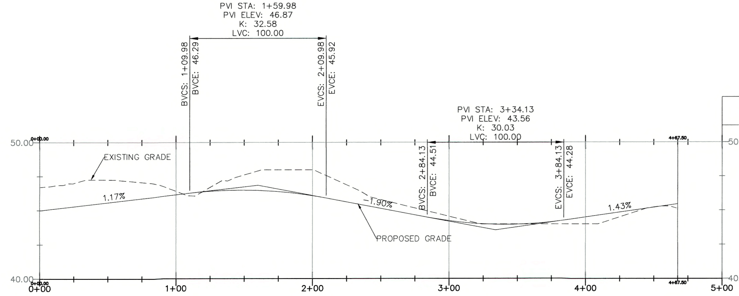
COLBY FARM LANE EXTENSION PROFILE
