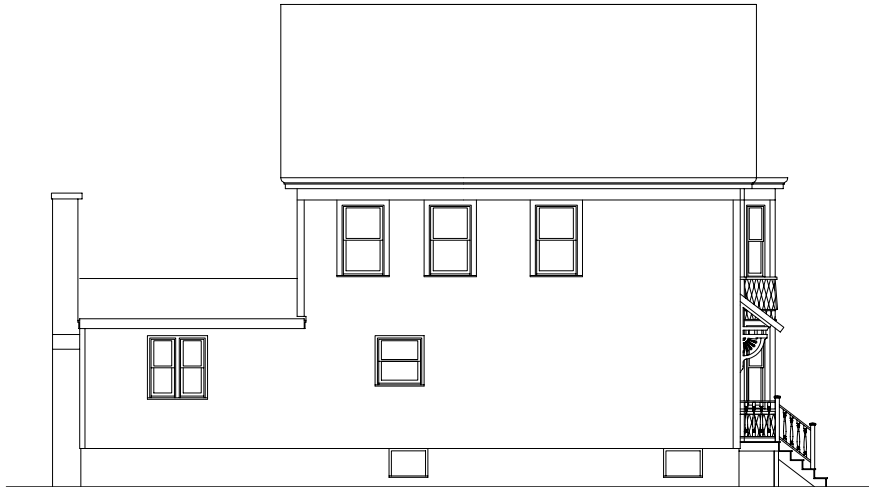
LEFT SIDE ELEVATION SCALE: 1/4" = 1'-0"
