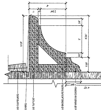
13 ORIGINAL WINDOW ENTABLATURE
